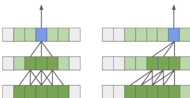
Figure 2: Standard Convolution Vs Causal Convolution [2]
